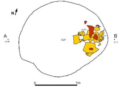
Cx 163 - plan intermediar/profil
